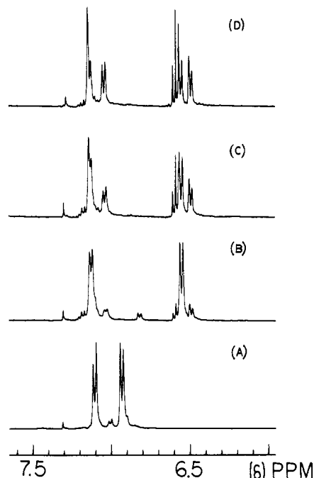
Figure 1. ^1\text{H} NMR spectra of [\text{C}_5(\text{CH}_3)_5]\text{Rh}[\text{P}(\text{CH}_3)_3](\text{H})(p\text{-C}_6\text{H}_4\text{CH}_3)\text{Br} in THF- d_6 : (A) after treatment with \text{AgPF}_6 at –40 °C; (B) after addition of 1 equiv of \text{Li}^+[\text{HB}(\text{s-Bu})_3]^- at –25 °C; (C) after 35 min at –10 °C; (D) after 110 min at +25 °C.
